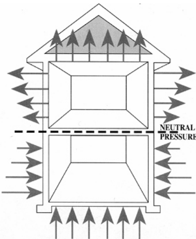
Figure 3. Stack-effect infiltration
