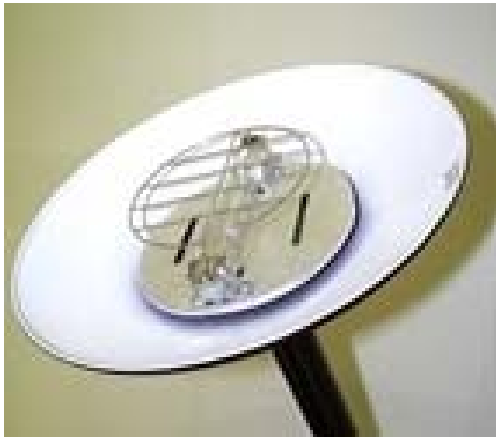
Source: Lighting Research Center 2000 Figure 19. Wire guard over 500 watt tubular halogen lamp
